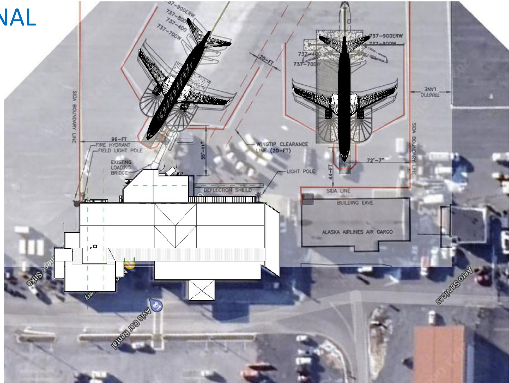
Existing Sitka Terminal and aircraft hardstands
